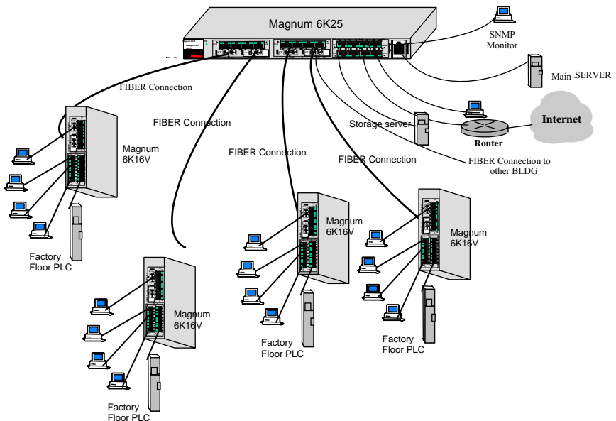
Fig. 2.1- The Industrial factory floor application with Magnum 6K16V
